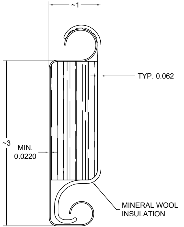
② SLAT DETAIL TYPICAL SECTION FRONT SLAT:
